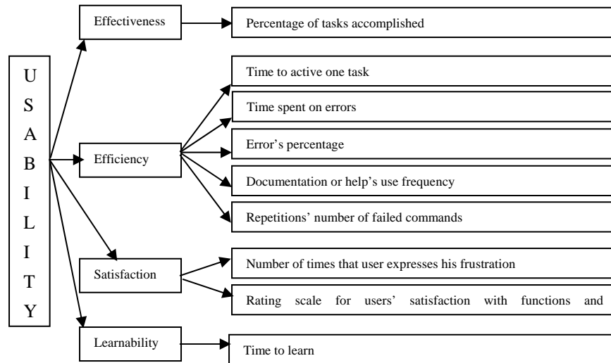
Figure 4: Usability Model (Dix et al. [4])
