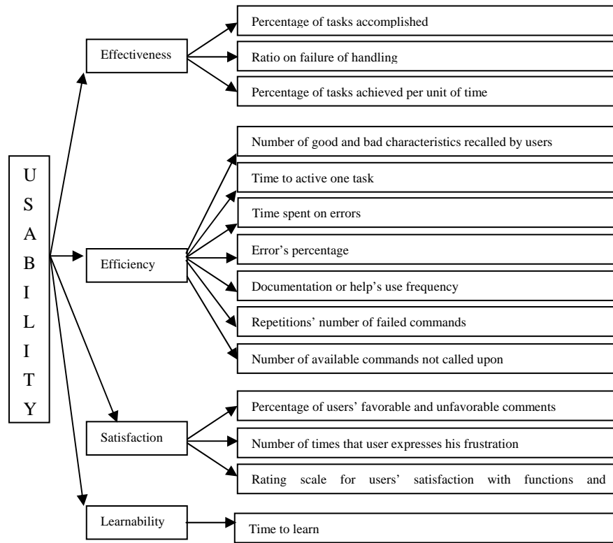
Figure 4: Usability Model (Dix et al. [4])
