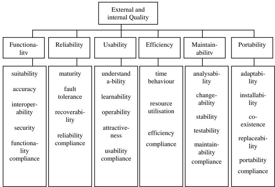
Figure 2: Software Quality – ISO 9126
