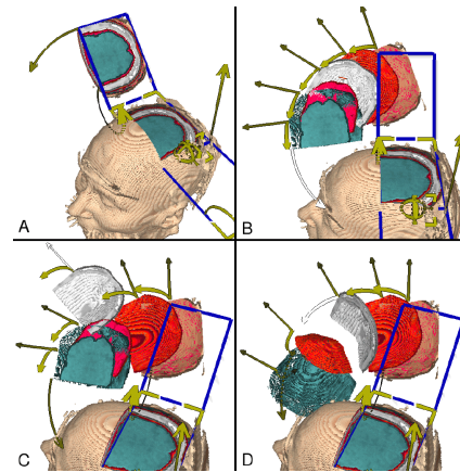
Figure 10: A: The left half of the Leafer hinges open the top of the head. B: The layers that make up the hinged-open region are fanned open. New widgets appear attached to each layer. C: A translation widget is used to pull out an individual layer. D: Rotation widgets are used to flip over layers.
