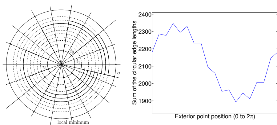
Fig. 4. Multi-modality of the function giving the sum of lengths. (Left) The construction of an example with 9 points – the radius r_k is given by r_0 + \delta + (k-1) \times \frac{r_{n+1} - r_0 - 2\delta}{n-1} . (Right) The corresponding sum of the circular edge lengths.
