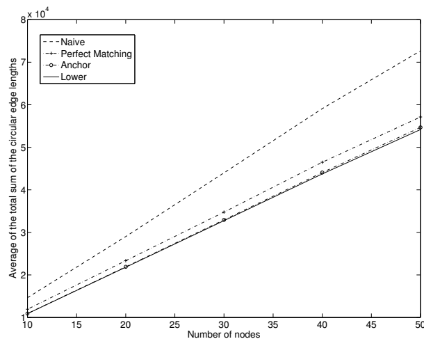
Fig. 8. Comparing the performance of the different algorithms on random bipartite graphs with n = 10, 20, 10, 40 and 50 nodes.
